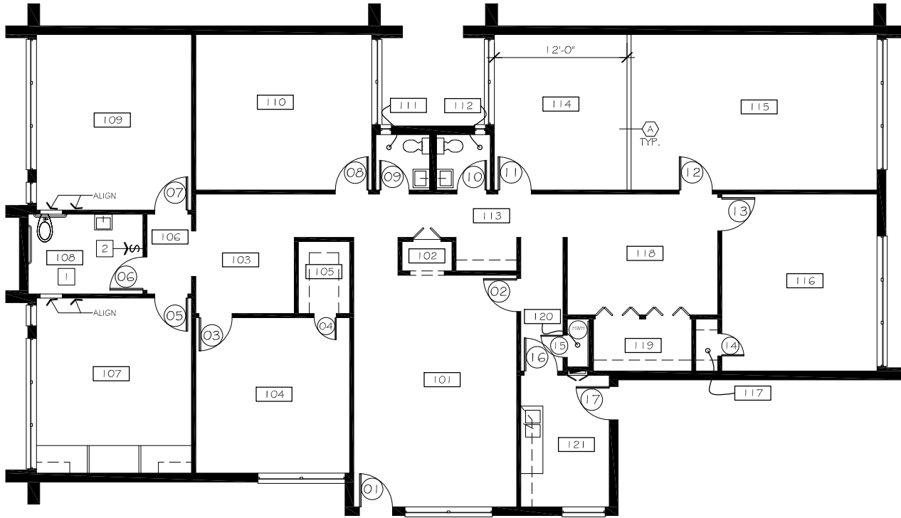
FIRST FLOOR - CONSTRUCTION PLAN SCALE: 1/8" = 1'-0"
