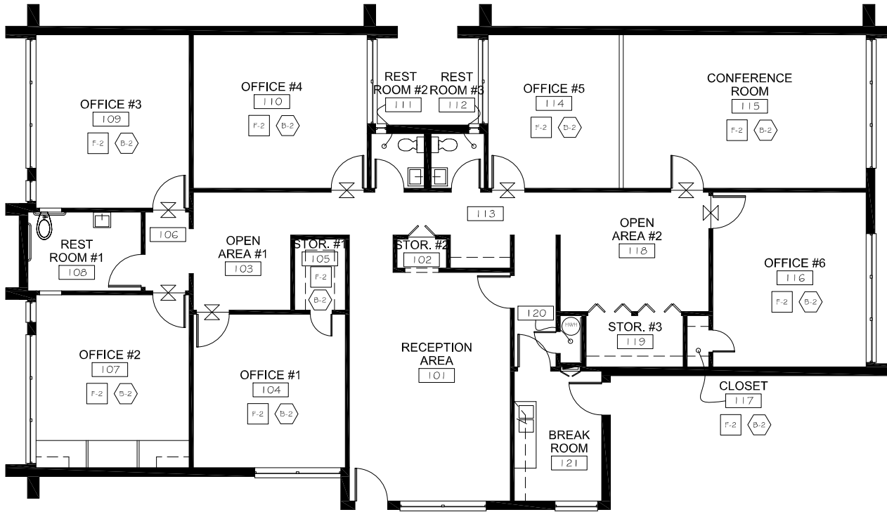
FIRST FLOOR - FINISH PLAN SCALE: 1/8" = 1'-0"
