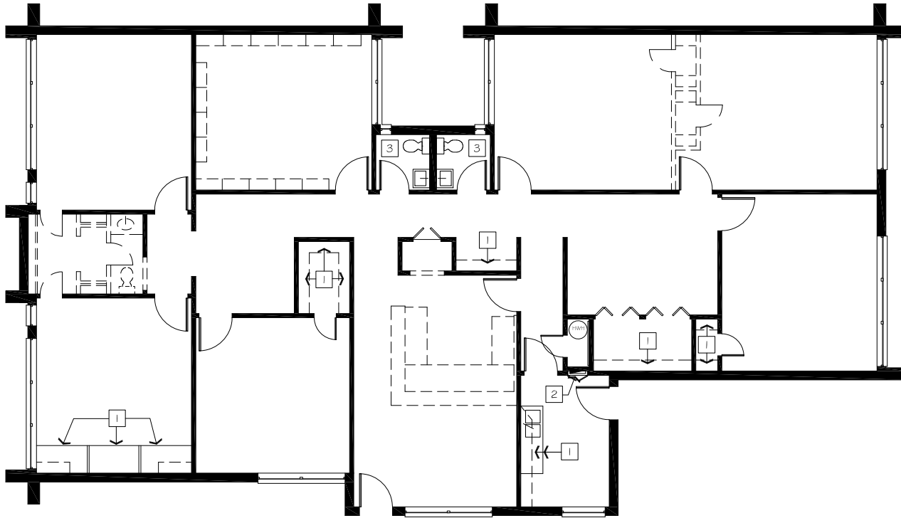
FIRST FLOOR - DEMOLITION PLAN SCALE: 1/8" = 1'-0"
